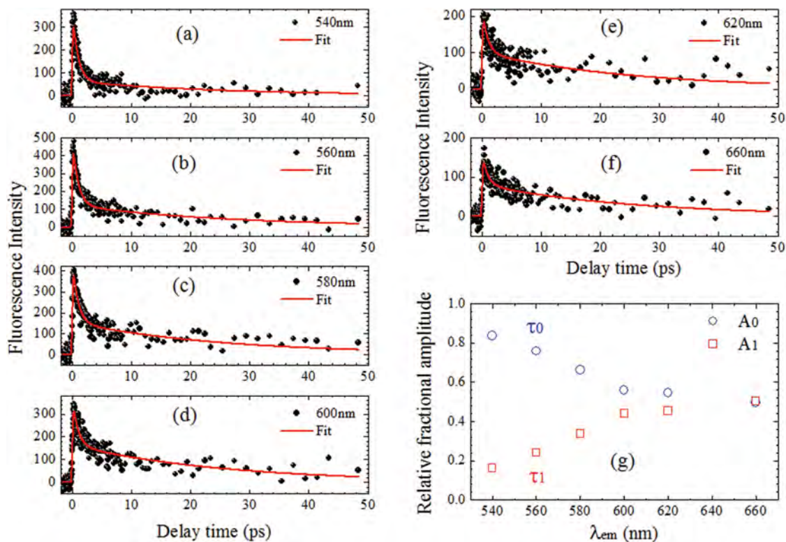
Figure 6 | (a–f) Fluorescence upconversion kinetics at \lambda_{\text{exc}}=400 nm and \lambda_{\text{em}} = 540\text{--}660 nm; (g) relative fractional amplitudes of two lifetime components ( \tau_0 = 0.9 \pm 0.2 ps; \tau_1 = 26 \pm 3 ps) versus wavelength.
